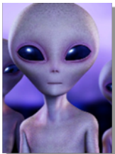
an alien
