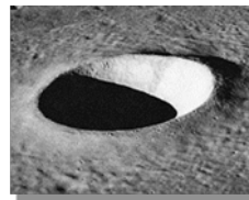
a crater
