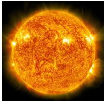
the Sun
